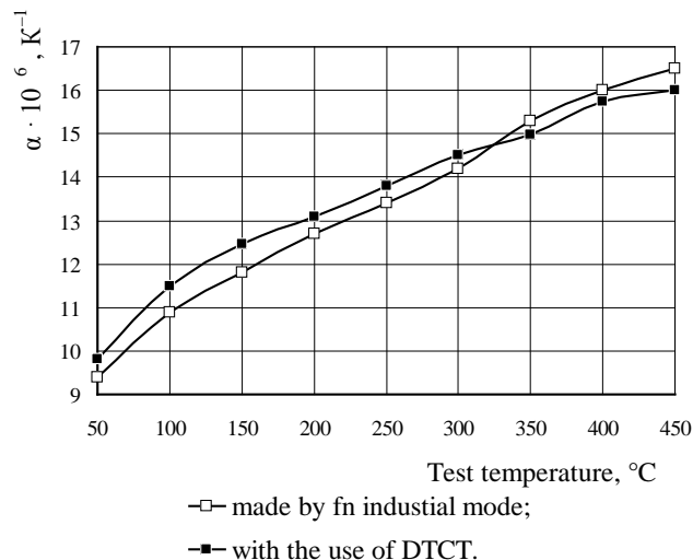
Fig.1 – Influence of thermal -cyclic forging on the linear expansion of hot- rolled sheet steel 10 (sheet thickness of 3mm)
