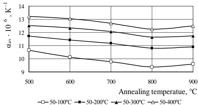
Fig. 4 – Influence of annealing temperature on average TCLE in various intervals of test temperatures of the sheet hot-rolled steel 10 made with use of DTCT
